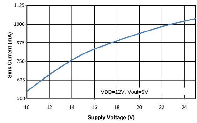
Figure 19. Output Sink Current vs. Supply Voltage
