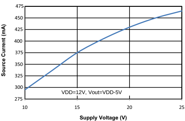
Figure 20. Output Source Current vs. Supply Voltage
